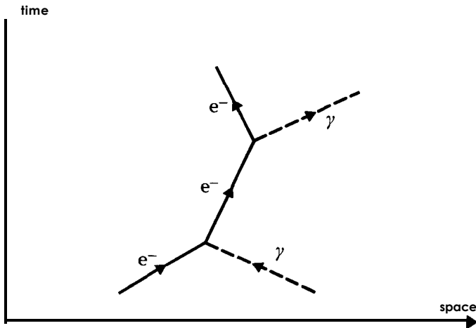
electron-photon scattering
